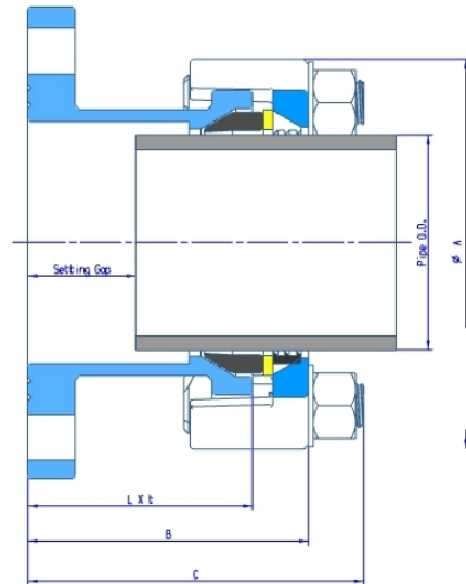
Plain End to Flange
